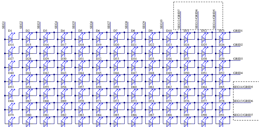
A diode needs to be connected in series for key/display multiplexing
