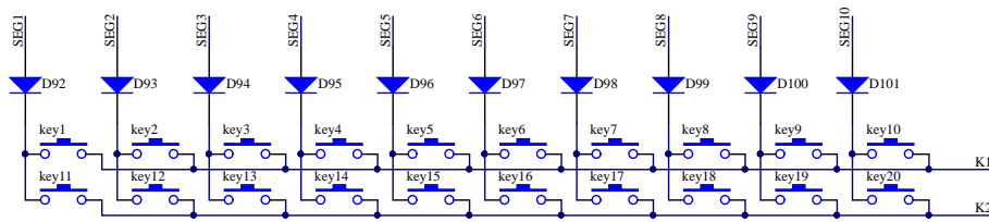
A diode needs to be connected in series for key/display multiplexing
